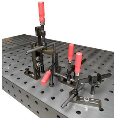
Images: Examples of use Clamping bolt with steel balls
